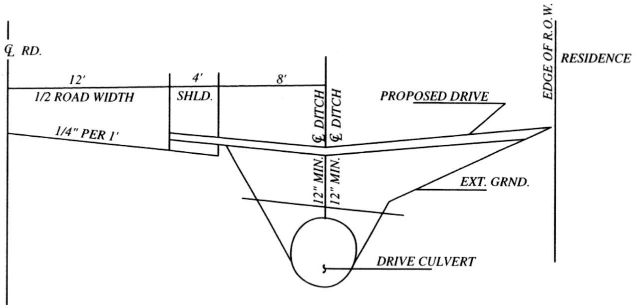
TYPICAL SECTION
